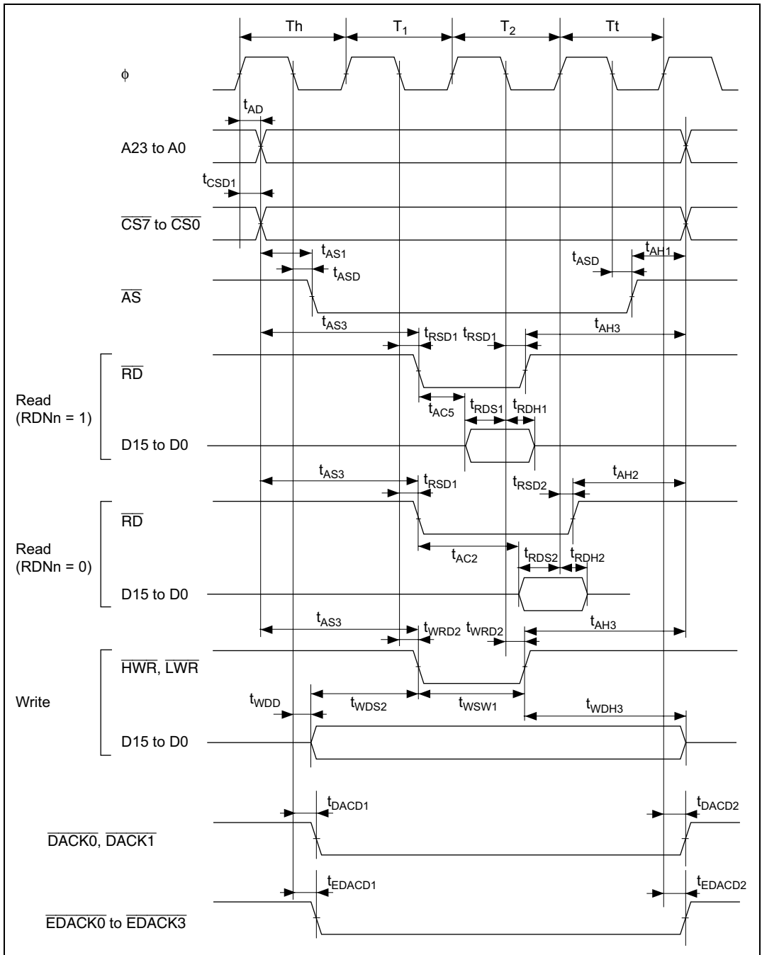
Figure 26.10 Basic Bus Timing: Two-State Access ( \overline{\text{CS}} Assertion Period Extended)
